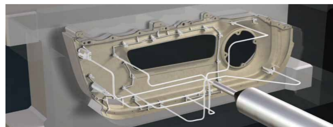
基材成形&樹脂成形(同時実施) Pressing base material and injection molding simultaneously
